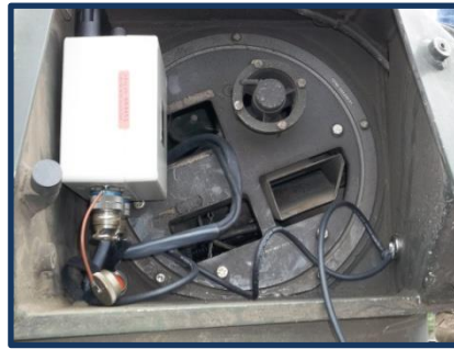
Step 2 – MOUNT THE FCIB IN THE 25MM LINK CHUTE AREA OF THE VEHICLE.
