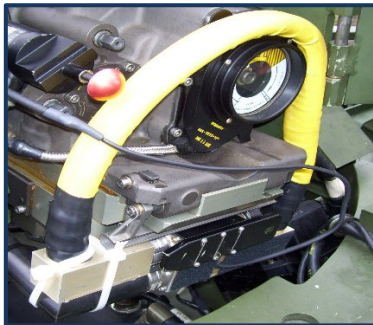
Step 1 – INSTALL THE HOM AND FCIB TO THE Mk44 CANNON.
