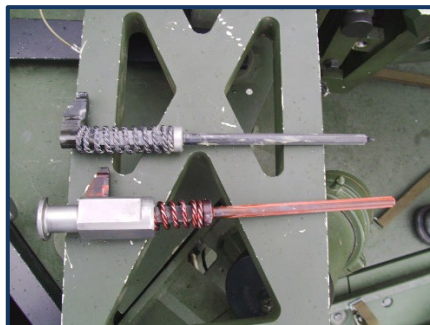
Step 2 – REPLACE THE Mk44 FIRING PIN WITH A DUMMY FIRING PIN.
