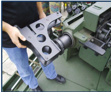
Step 3 – INSTALL GTS-30 MOUNT ASSEMBLY INTO Mk44 CANNON.
